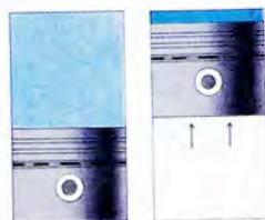
Before / After the mixture has been compressed
