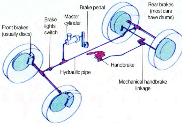
Braking system
