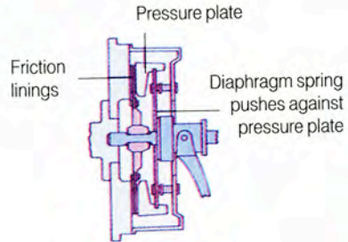
Clutch engaged
