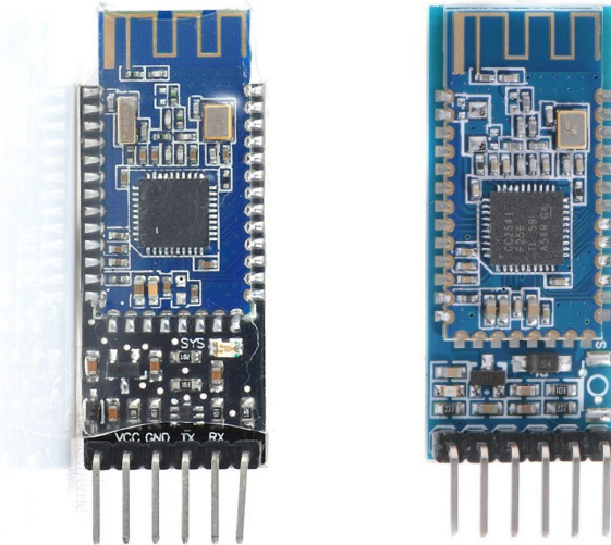
Εικόνα 80: Οι μονάδες BLE HM-10 (αριστερά) και AT-09 (δεξιά)
